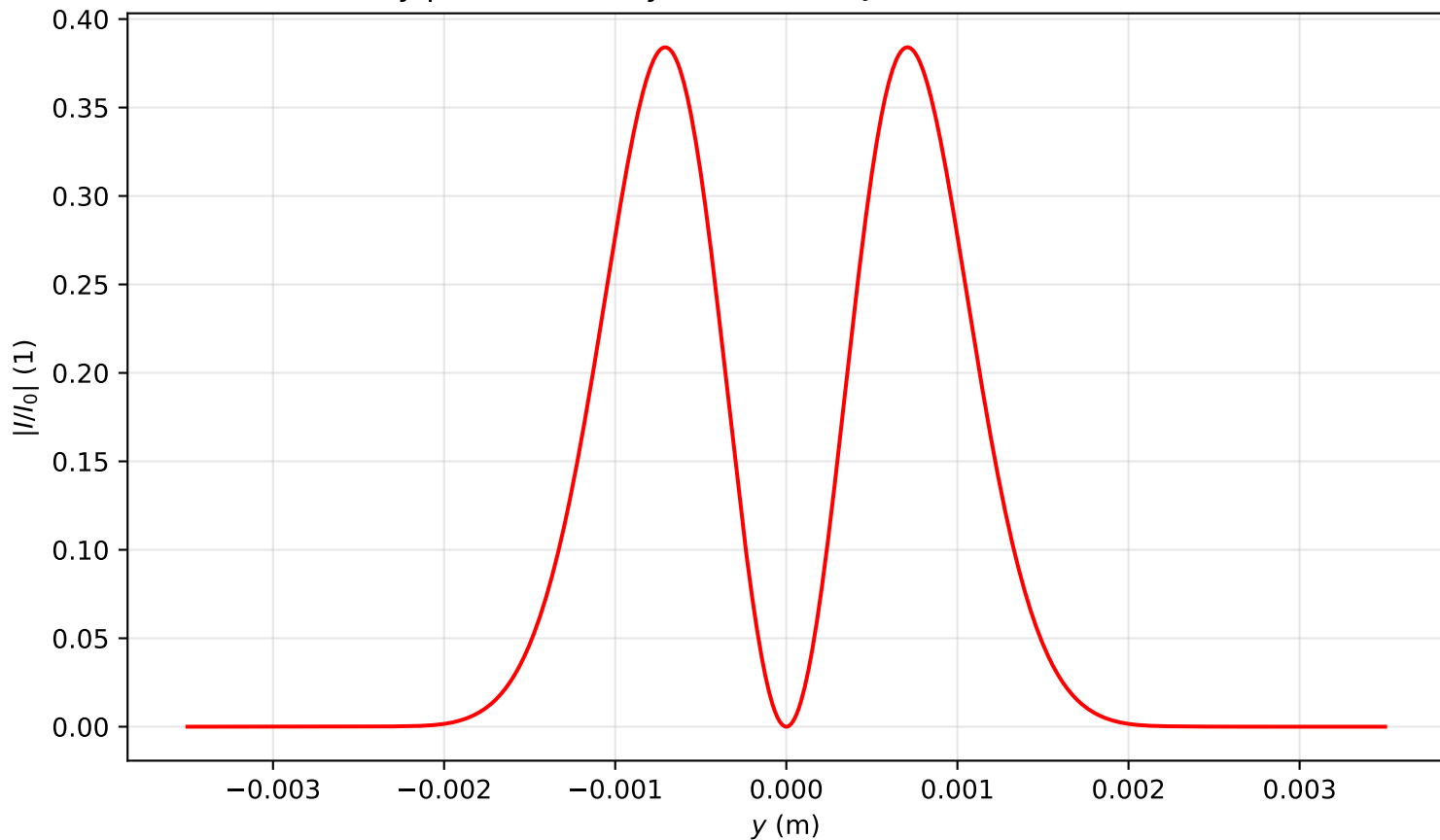
Intensity profile I(x=0, y, z=2.070)/I_0 , P_{in}=0.5P_{cr} , artificial time
